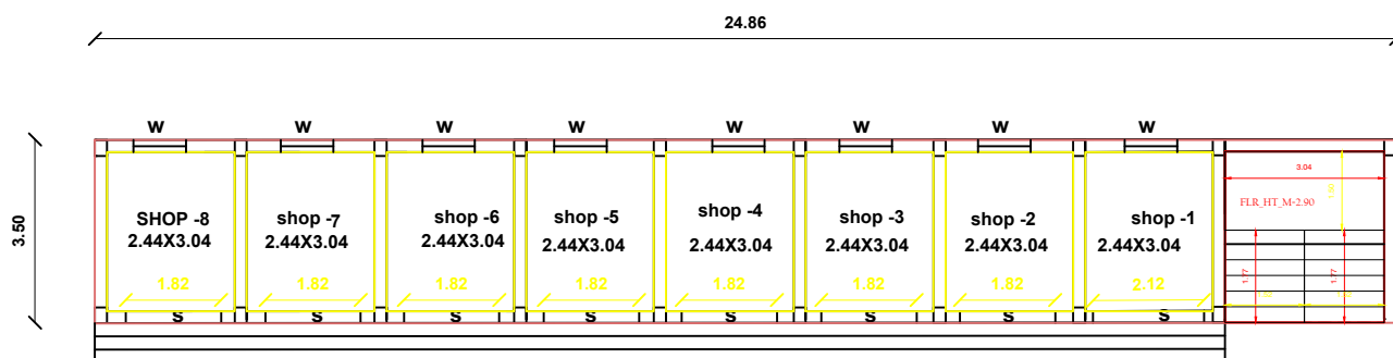
G.FLOOR PLAN
