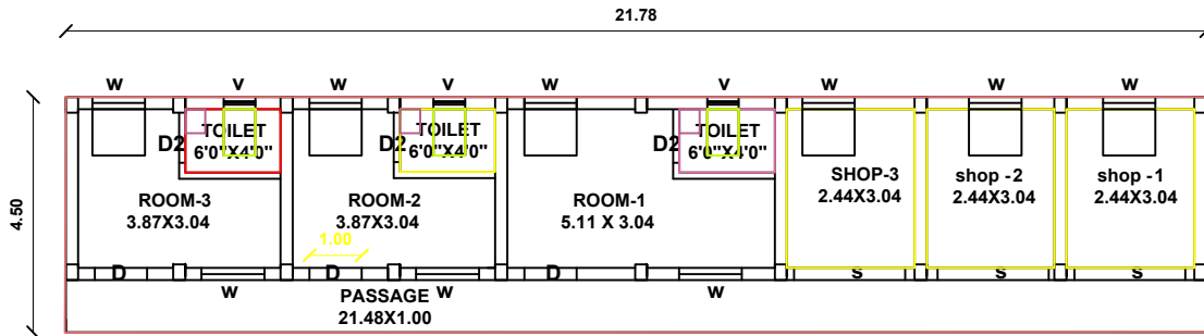
F.FLOOR PLAN
