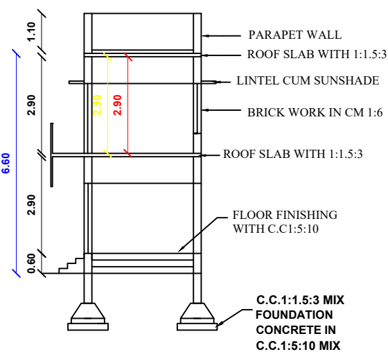
SECTION ON G1G2"
