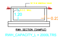
RWH_SECTION (SAMPLE) RWH_CAPACITY_L = 2000LTRS
