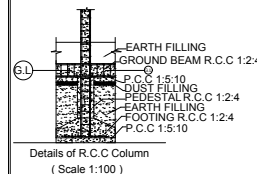
Details of R.C.C. Column (Scale 1:100)
