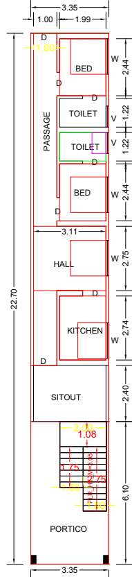
G.F. PLAN
