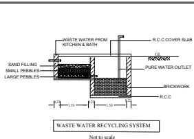
WASTE WATER RECYCLING SYSTEM Not to scale
