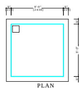
DETAILS OF COLLECTION SUMP FOR RAIN WATER HARVESTING OF ROOF TOP RAIN WATER RWV_CAPACITY_L=5000LTRS
