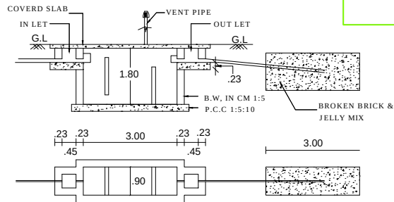
PLAN & SECTION OF SEPTIC TANK & TRENCH
