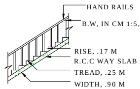
SECTION ON STAIR
