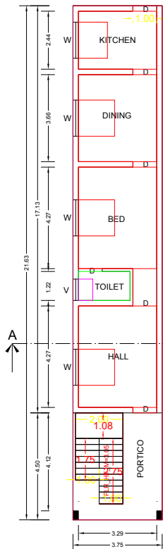
G.F. PLAN
