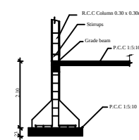
Column Detail
