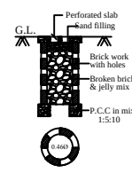
PERCOLATION PIT (NOT FOR SCALE)
