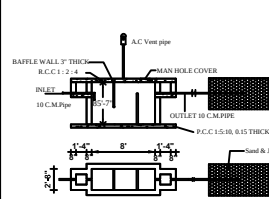
Septic tank and trench
