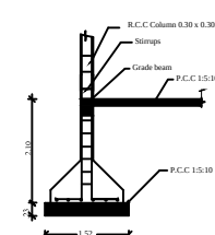
Column Detail
