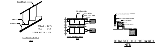
DETAILS OF FILTER BED & WELL
