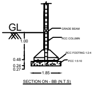
SECTION ON - BB (NTS)
