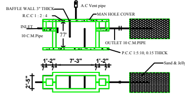
Septic tank and trench
