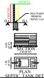
PLAN SEPTIC TANK DETAILS
