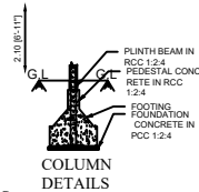
COLUMN DETAILS
