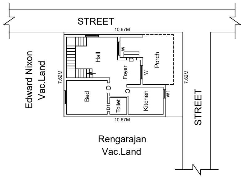
SITE PLAN
