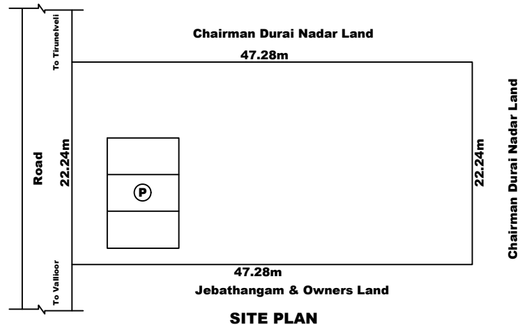
SITE PLAN
