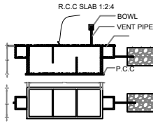
SEPTIC TANK AND TRENCH NTS
