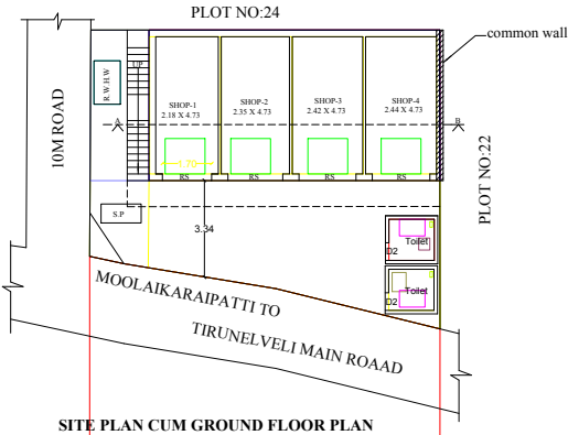
SITE PLAN CUM GROUND FLOOR PLAN
