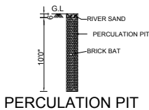
PERCOLATION PIT
