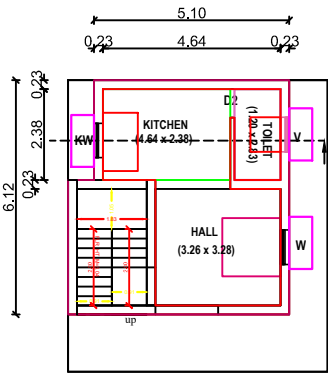
PROPOSED SECOND FLOOR PLAN
