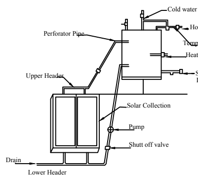
Details Of Solar Water Heater (NTS)
