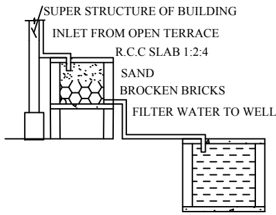
Rainwater harvesting
