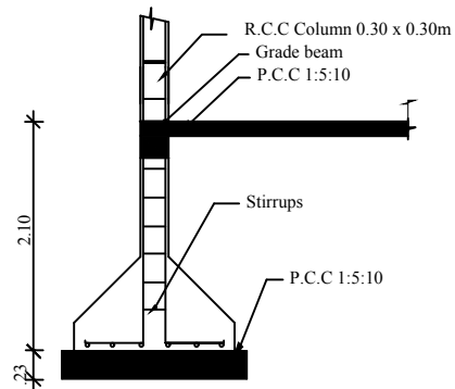
Column Detail
