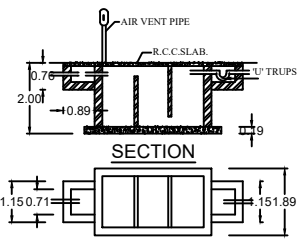
SEPTIC TANK PLAN
