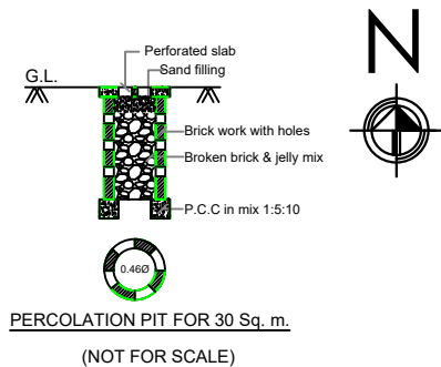
PERCOLATION PIT FOR 30 Sq. m.
