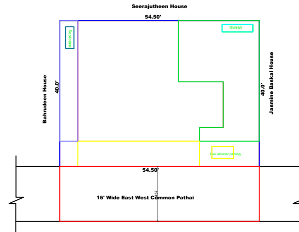
SITE PLAN
