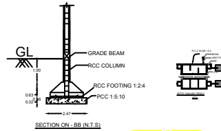
SECTION ON - BB (IN T.S.)
