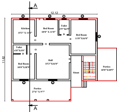
EXG.GROUND FLOOR PLAN
