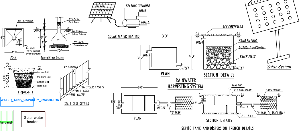
SEPTIC TANK AND DISPERSION TRENCH DETAILS
