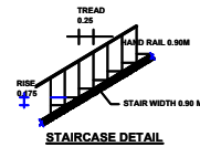
STAIRCASE DETAIL
