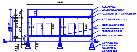
SECTION ON G1G2"
