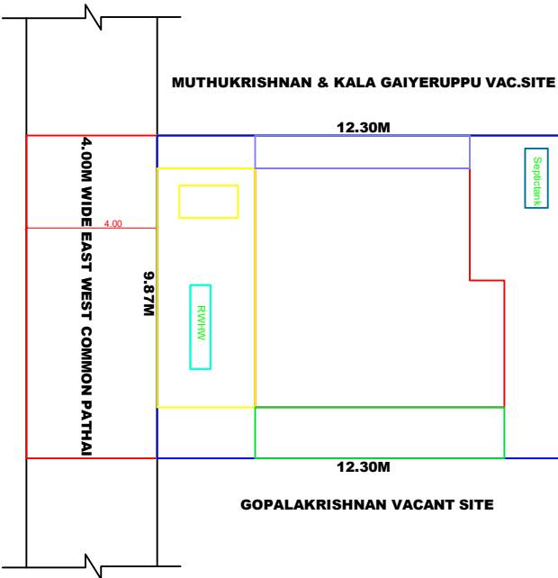
SITE PLAN
