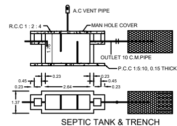
SEPTIC TANK &amp; TRENCH
