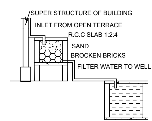
RAINWATER HARVESTING
