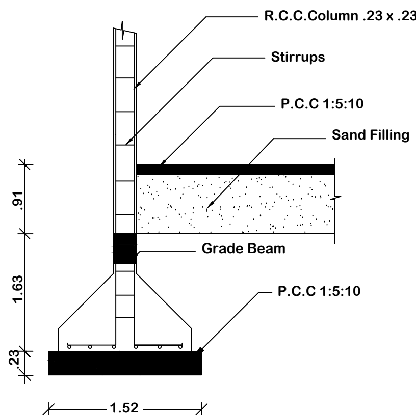
COLUMN DETAIL
