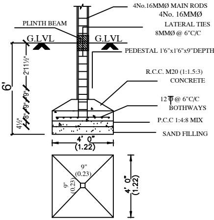
FOUNDATION DETAIL
