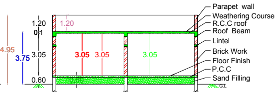
SECTION AB
