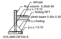
COLUMN DETAILS
