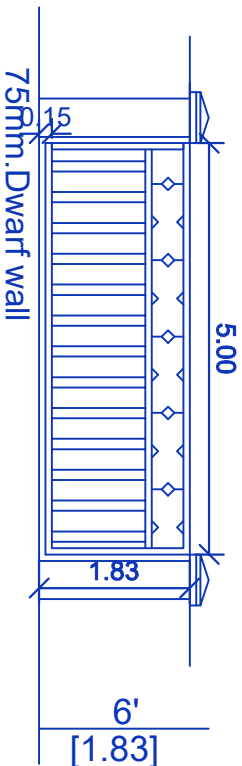
DETAILS OF COLLECTION SUMP FOR RAIN WATER HARVESTING OF ROOF TOP RAIN WATER RWH_CAPACITY_L=5000LTRS
