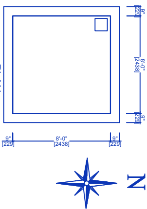
DETAILS OF COLLECTION SUMP FOR RAIN WATER HARVESTING OF ROOF TOP RAIN WATER RWH_CAPACITY_L=5000LTRS
