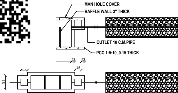
SEPTIC TANK & TRENCH
