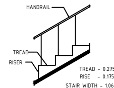
STAIRCASE DETAILS NTS
