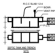
SEPTIC TANK AND TRENCH NTS
