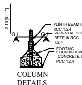
COLUMN DETAILS
