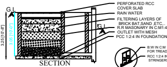
RAIN WATER HARVESTING OF RECHARGE TRENCH METHOD
