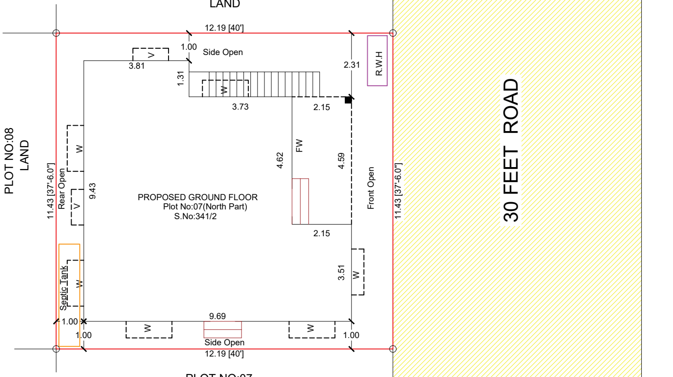
PLOT NO:07 South Part LAND SITE PLAN (Scale 1:100)
