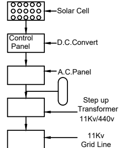
SOLAR SYSTEM FLOW DIAGRAM.
