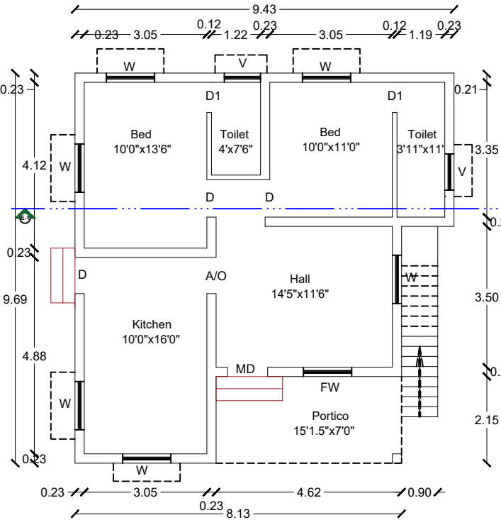
PRO-GROUND FLOOR
