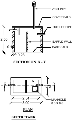
SEPTIC TANK
