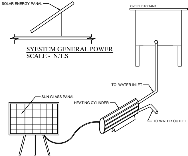
SOLAR WATER HEATING SYSTEM SCALE - N.T.S
