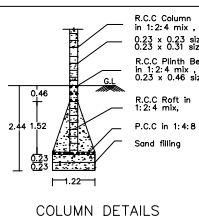
COLUMN DETAILS
