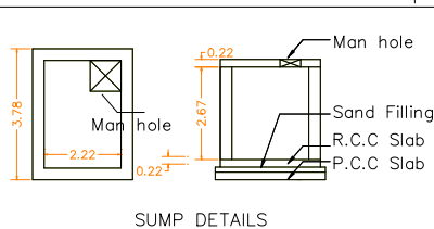
SUMP DETAILS
