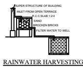
RAINWATER HARVESTING
