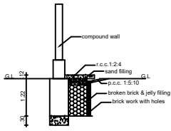
PLINTH BOUNDARY PERCOLATION PIT
