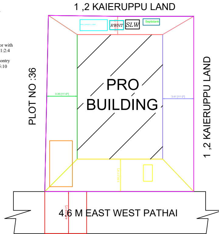
SITE PLAN
