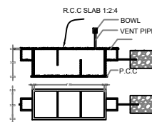
SEPTIC TANK AND TRENCH NTS
