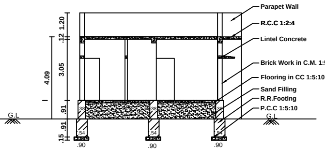
SECTION "AB"
