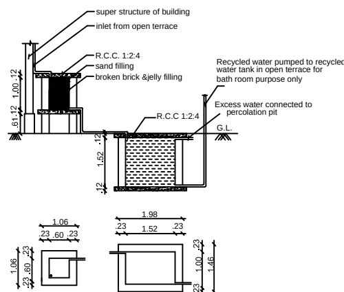
Sump and Filter Bed
