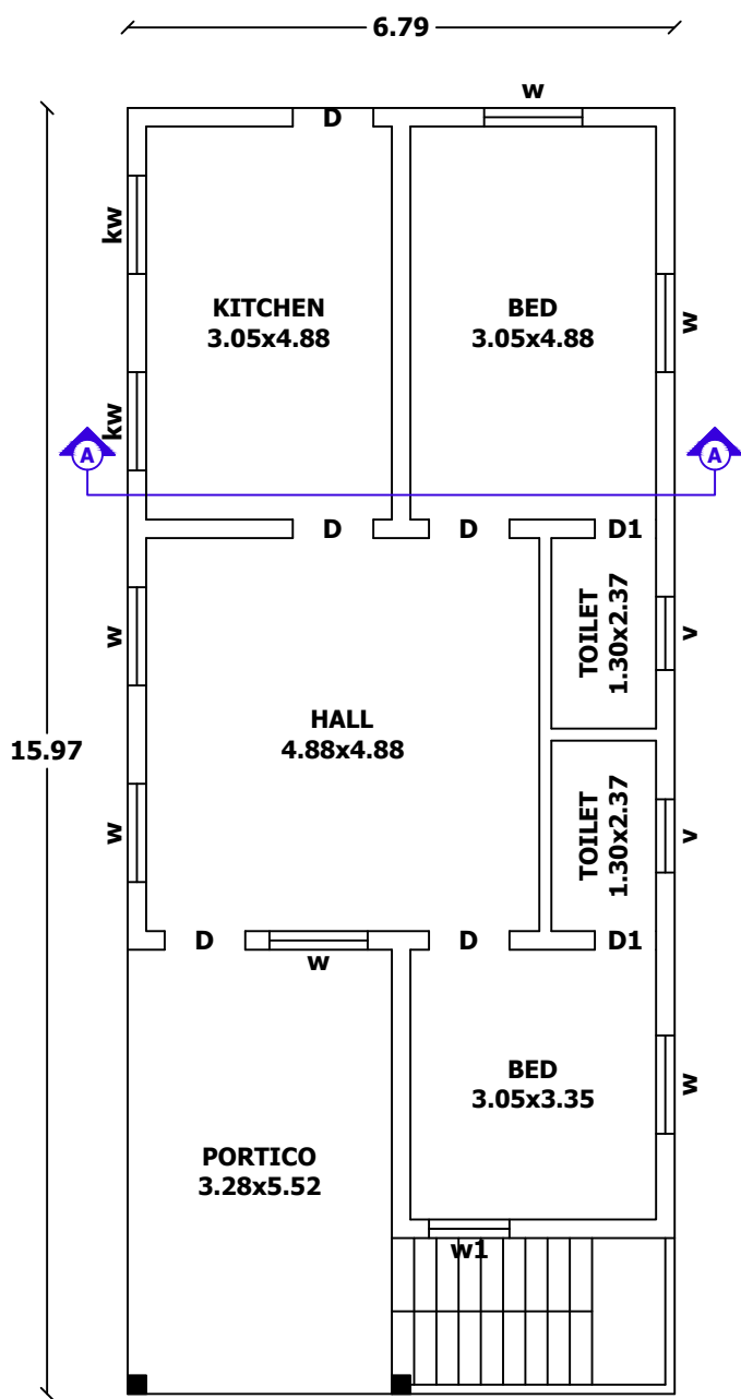
PLAN
