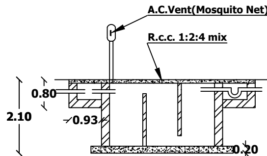
SECTION
