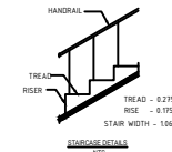
STAIRCASE DETAILS
