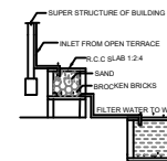
DETAILS OF FILTER BED & WELL NTS
