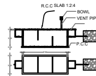
SEPTIC TANK AND TRENCH NTS
