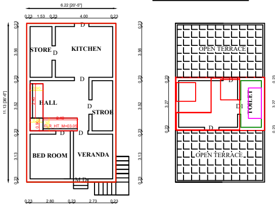
EXG.GROUND FLOOR PLAN
