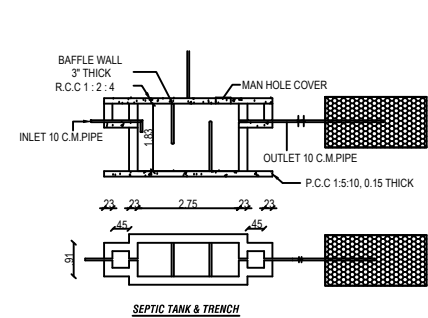
SEPTIC TANK & TRENCH
