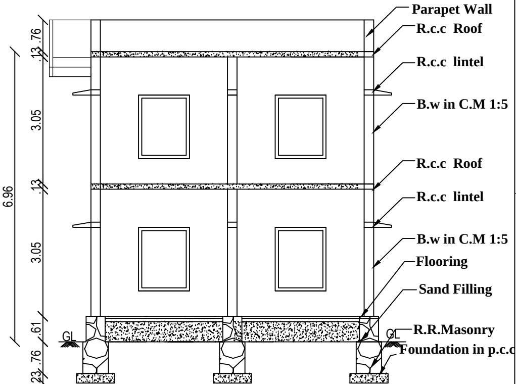
SECTION-AB
