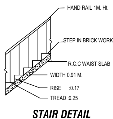
STAIR DETAIL
