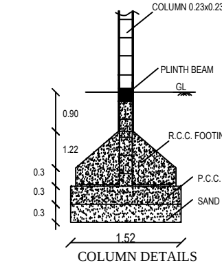
COLUMN DETAILS
