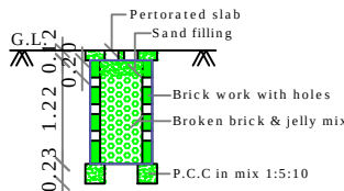
PERCOLATION PIT FOR 30 Sq. m. (Scale:- 1:50)
