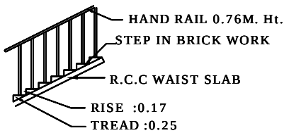
STAIR CASE DETAIL
