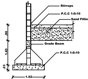
COLUMN DETAIL
