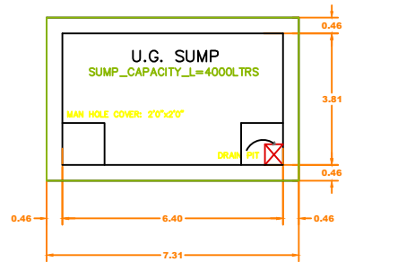
SUMP DETAIL
