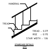
STAIRCASE DETAILS
