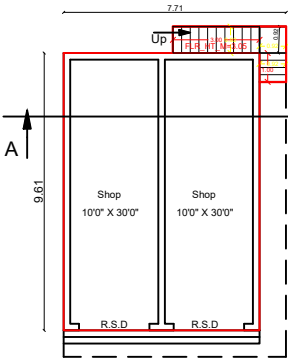
EXG.GROUND FLOOR PLAN
