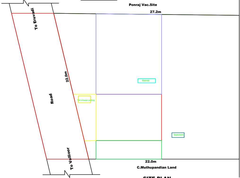
SITE PLAN
