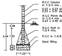
COLUMN DETAILS
