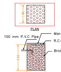
RAINWATER COLLECTION TANK
