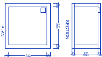
DETAILS OF COLLECTION SLUMP FOR RAIN WATER HARVESTING OF ROOF TOP RAIN WATER
