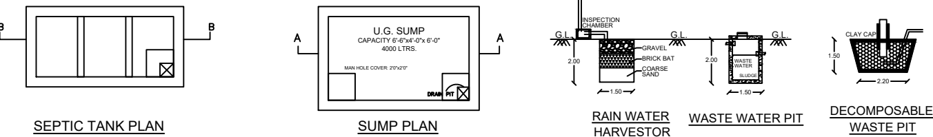
SEPTIC TANK PLAN
