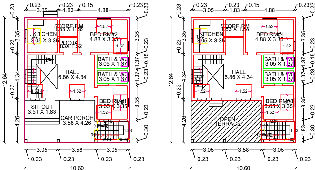
Prop. GROUND FLOOR PLAN
