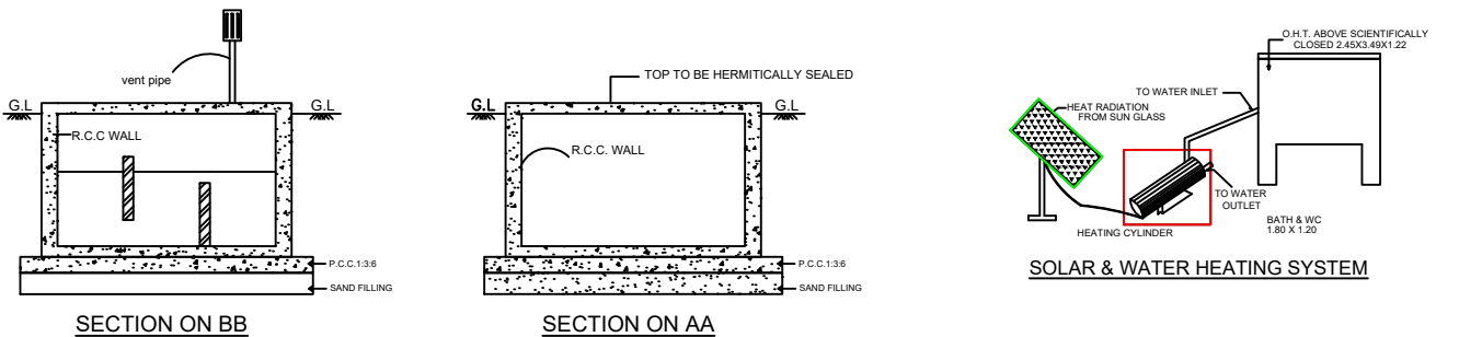
SECTION ON BB
