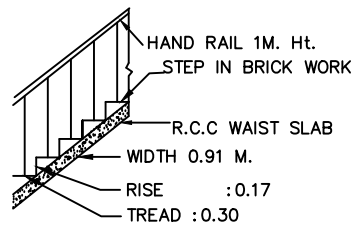
STAIR DETAIL
