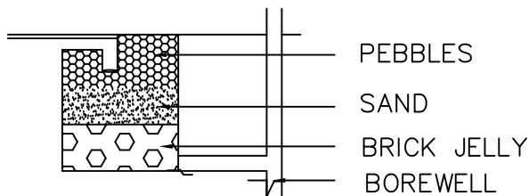
RAINWATER FILTRATION
