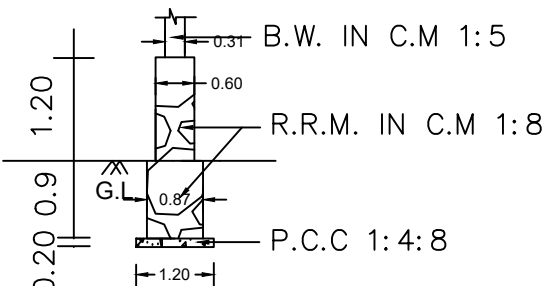
COLUMN DETAILS
