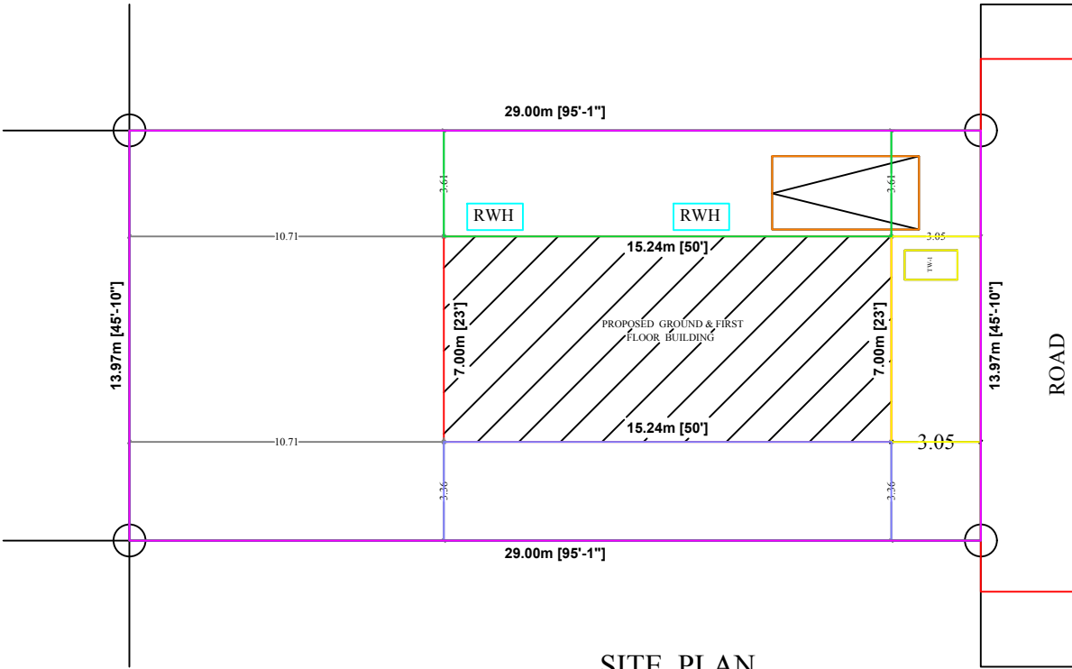
SITE PLAN
