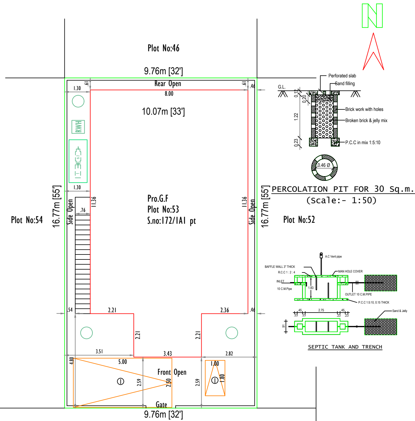
RAINWATER HARVESTING
