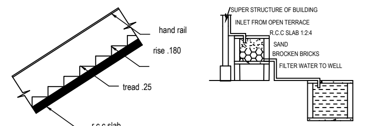
RAINWATER HARVESTING
