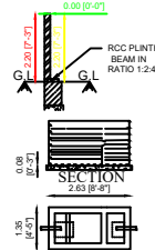
SEPTIC TANK DETAILS
